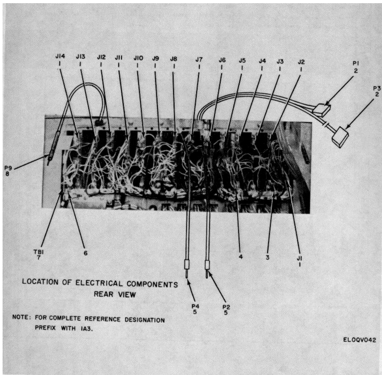
Figure 25. Sensing and Control Shelf (1A3), AN/FRC-80(V)1, Rear View.
