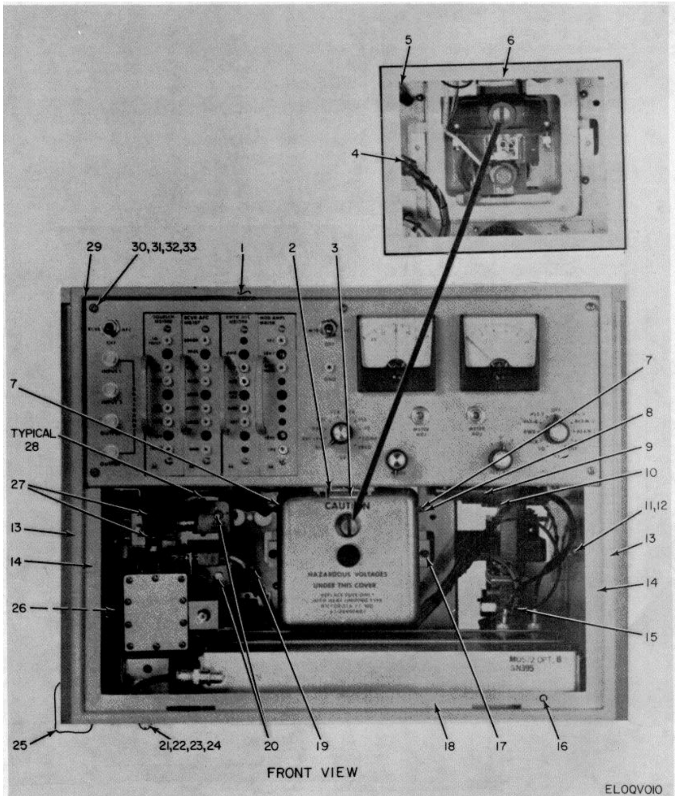
Figure 5. Receiver-Transmitter Radio RT-986(P)/FRC (1A1), Mounting Hardware (Sheet 1 of 2).
