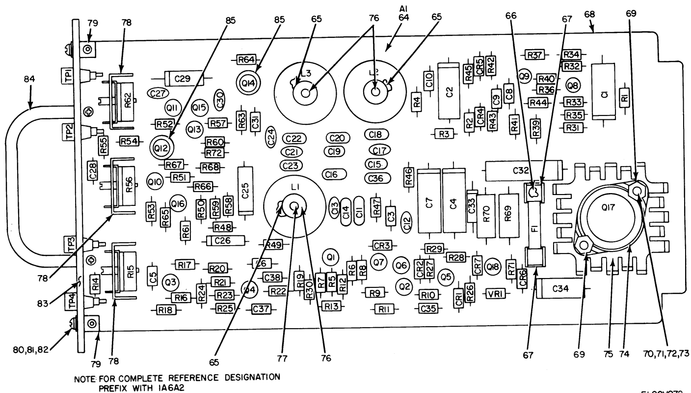
Figure 43. Transmitter, Orderwire T-1162/FRC (1A6A2) (Sheet 1 of 3).
