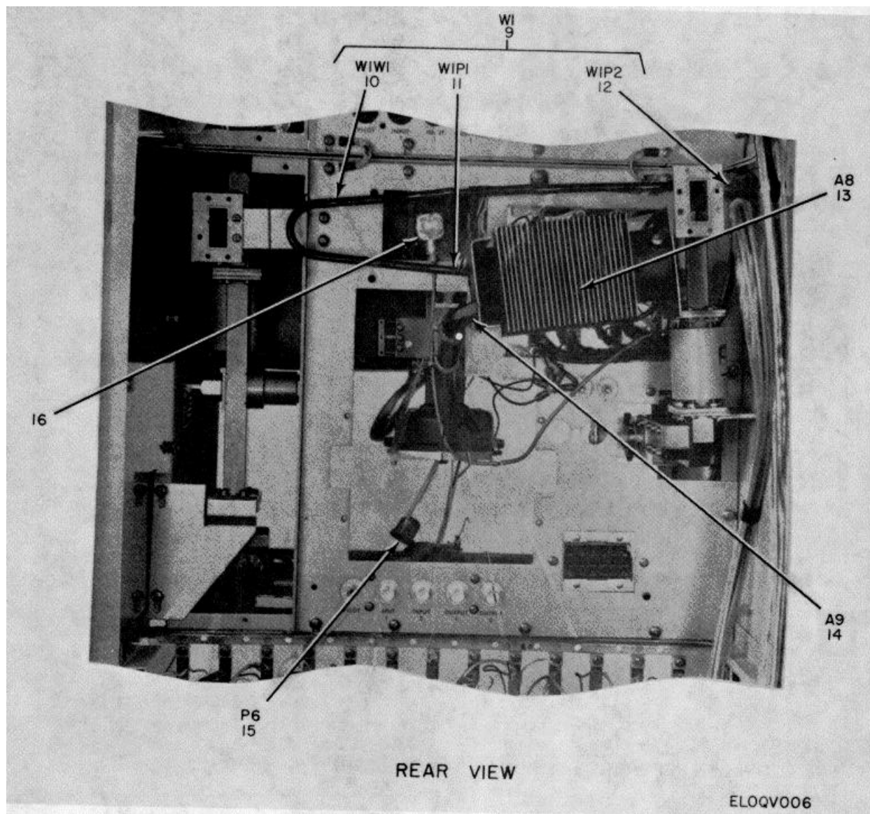
Figure 3. Receiver-Transmitter Radio RT-986(P)/FRC (1A1) (Sheet 2 of 2).
