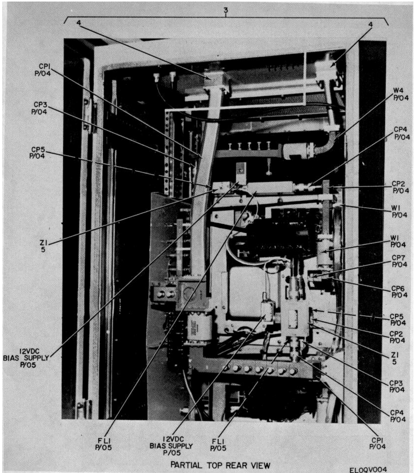
Figure 2. Radio Set AN/FRC-80(V)3 (1) (Sheet 2 of 2)
