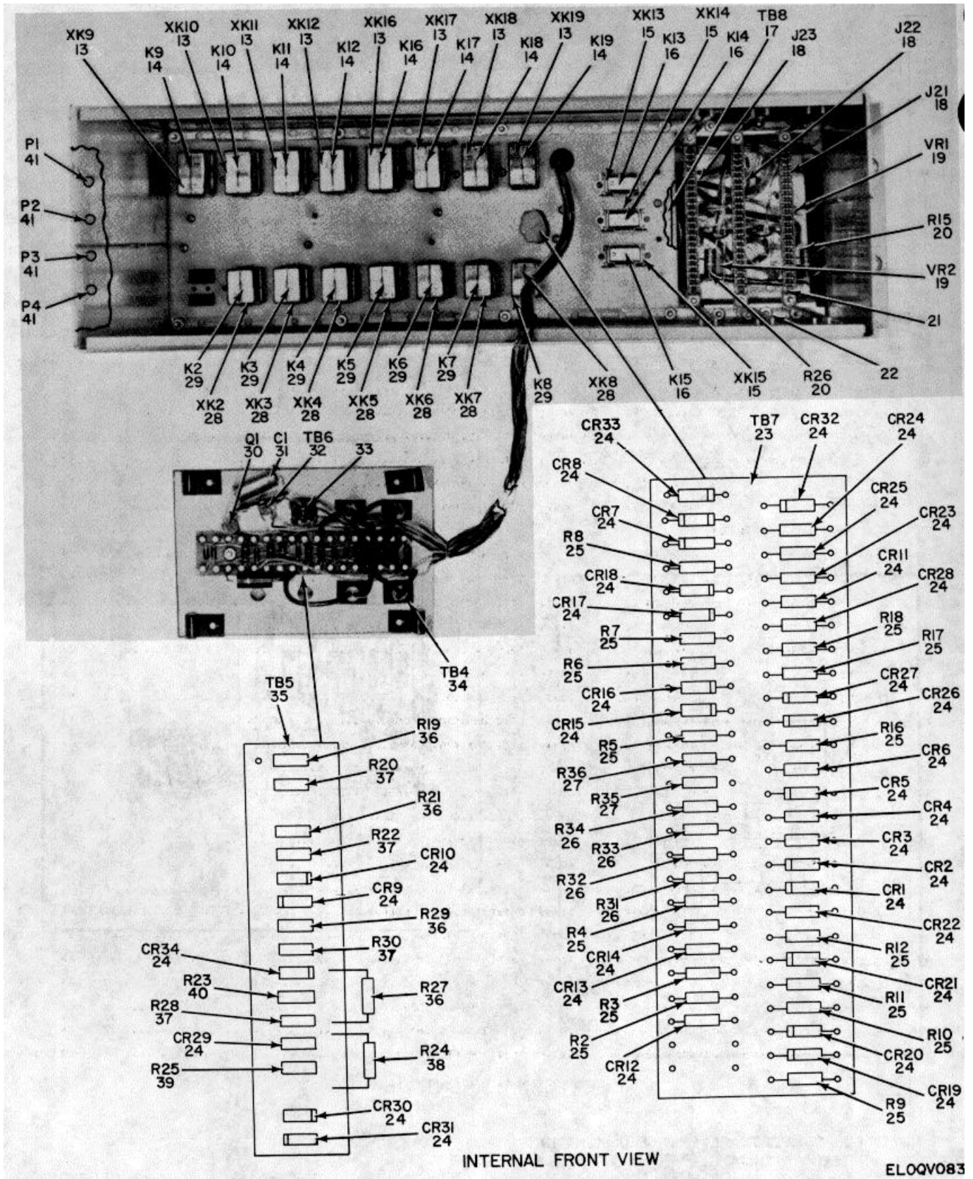
Figure 49. Panel, Combiner Bypass and Alarm SB-3428/FRC (1A7) (Sheet 2 of 2).
