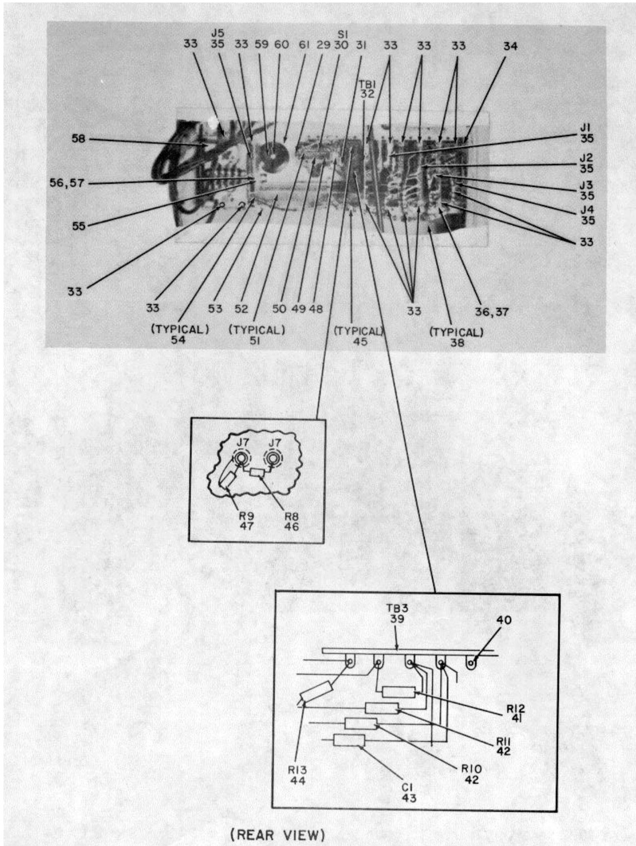
Figure 40. Receiver/Transmitter, Orderwire RT-987(V)1/FRC (1A6) (Sheet 2 of 2).
