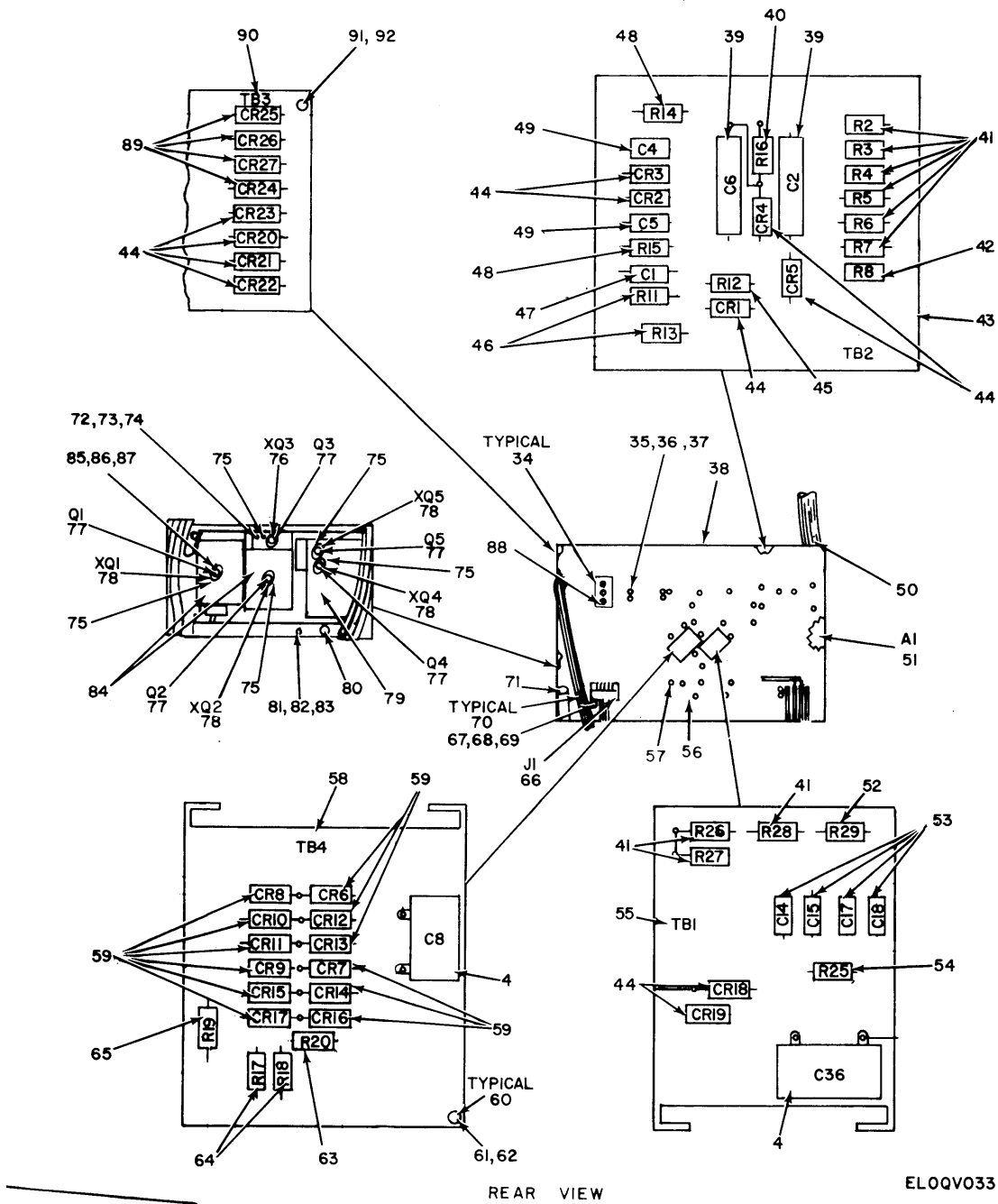
Figure 18. Power Supply PP-6414/FRC (1A2A1) (Sheet 2 of 2).
