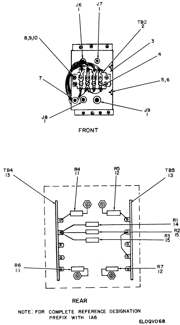
Figure 41. Receiver/Transmitter, Orderwire RT-987(V)1/FRC (1A6), Bracket Assembly.
