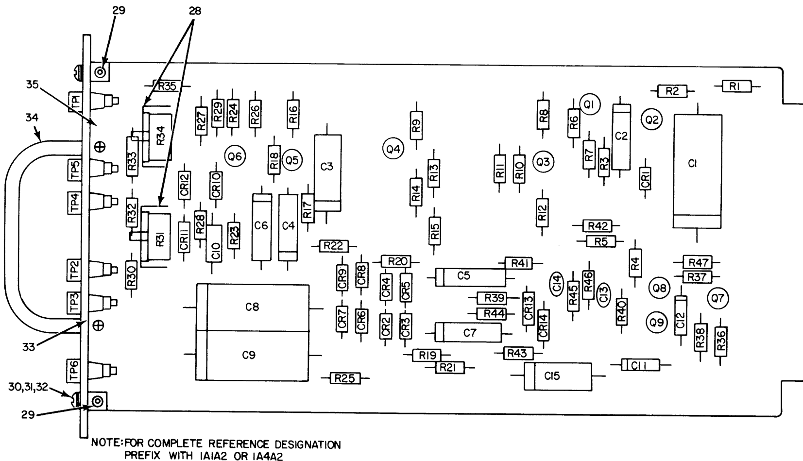
Figure 8. Control, Receiver C-8434/FRC (1A1A2) (Sheet 1 of 2).
