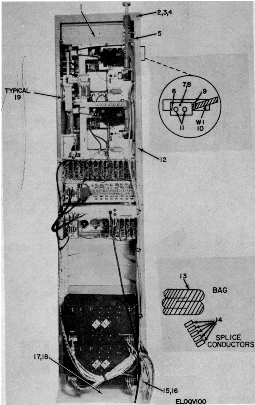
Figure 62. Rack Assembly, Electrical Equipment MT-4247/FRC.
