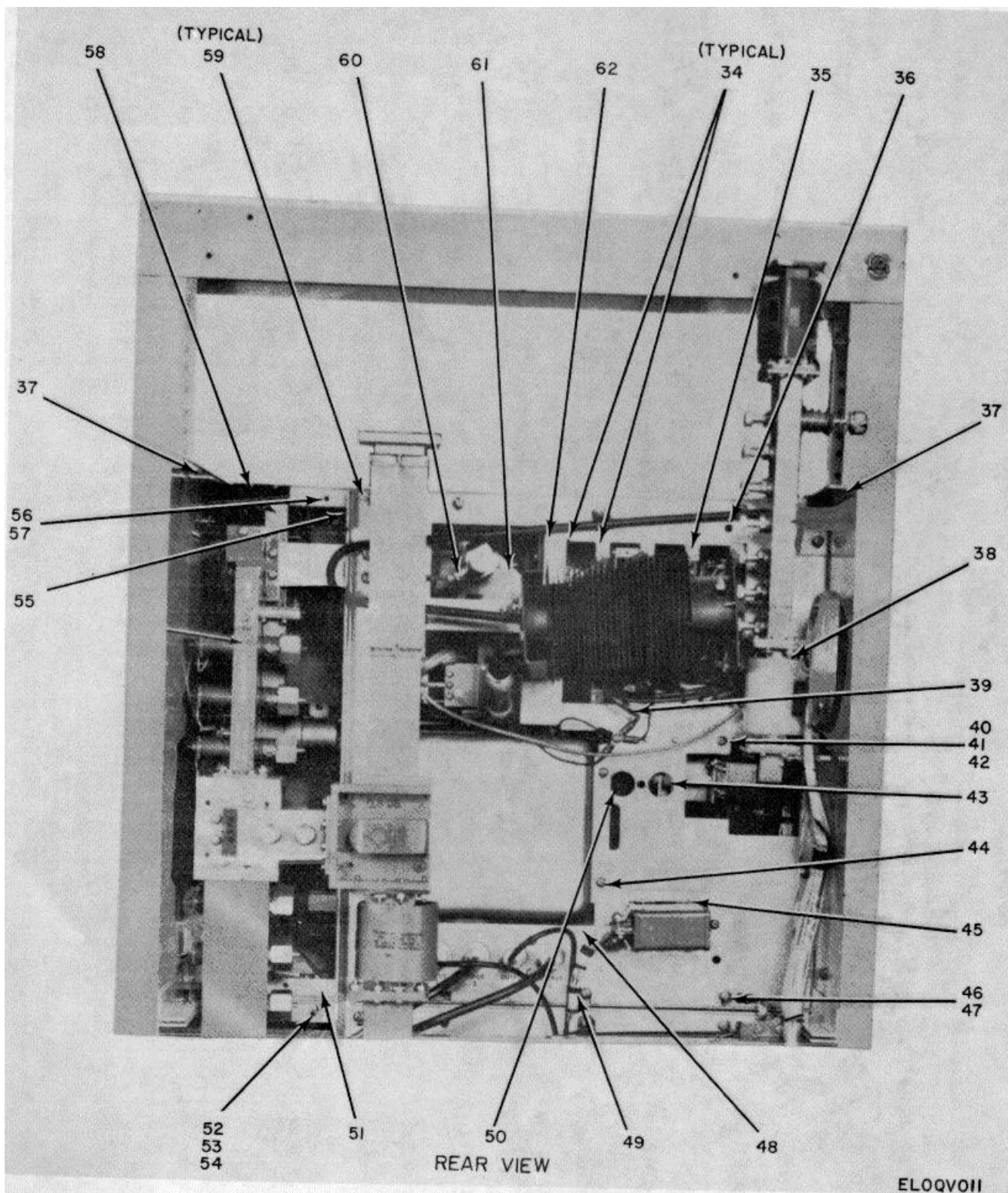
Figure 5. Receiver-Transmitter Radio RT-986(P)/FRC (1A1), Mounting Hardware (Sheet 2 of 2).
