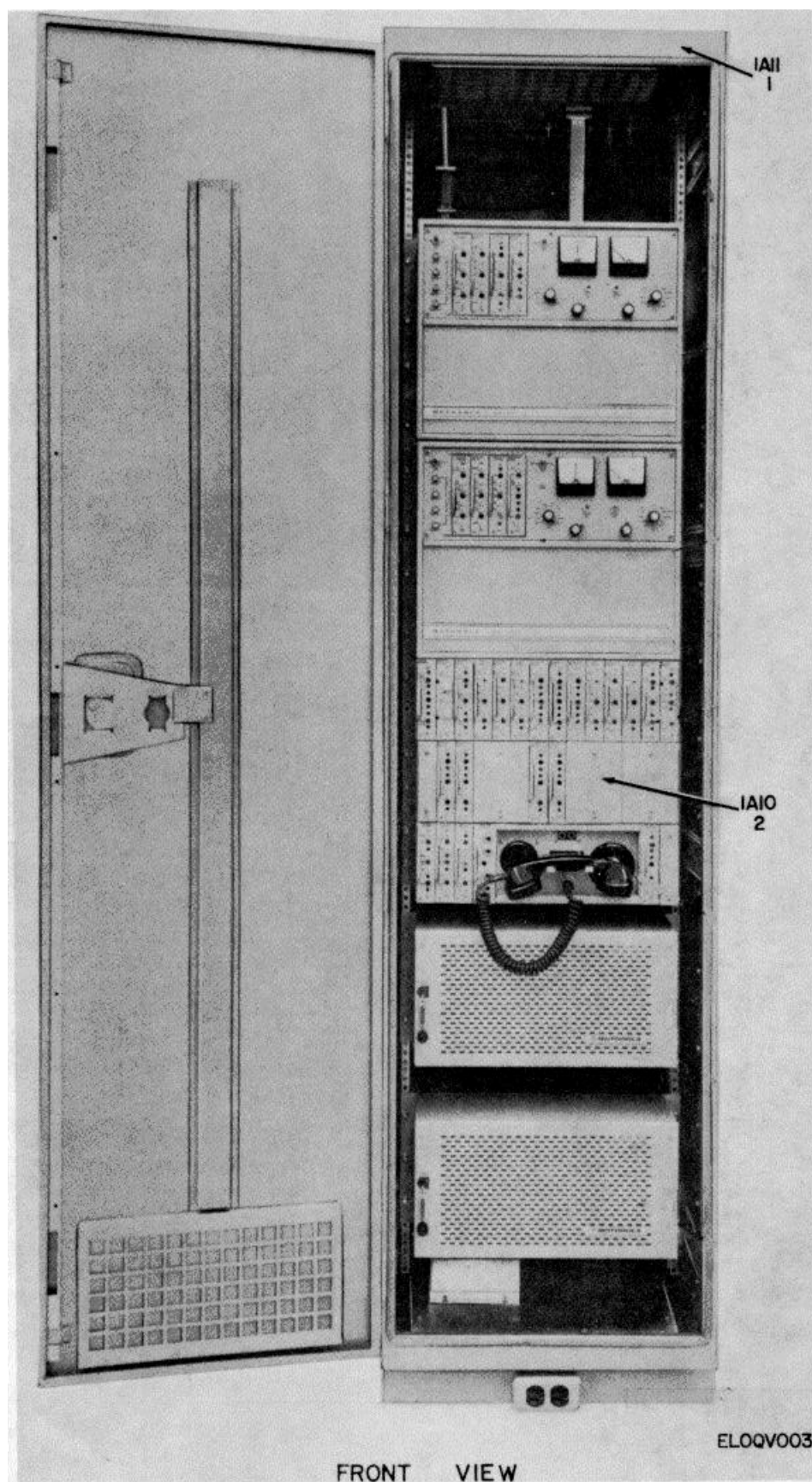
Figure 2. Radio Set AN/FRC-80[V]3 (1) (Sheet 1 of 2).
