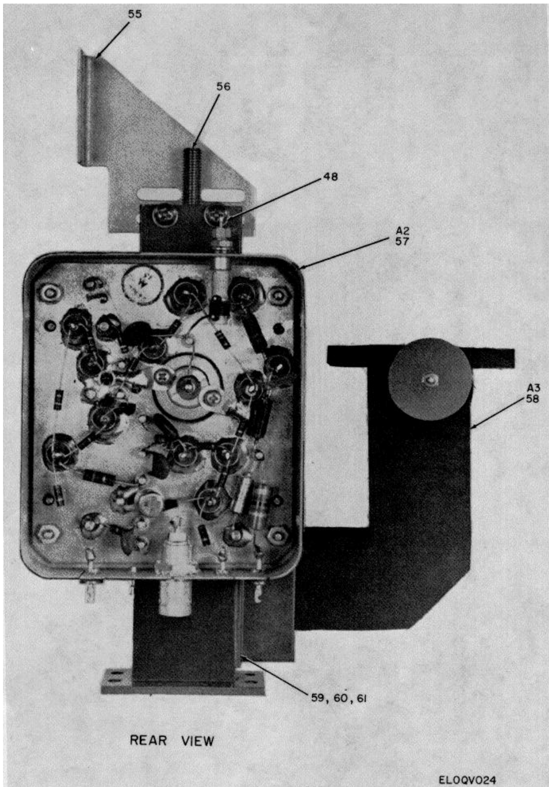
Figure 11. Mixer-Local Oscillator-Preamp (1A1A7) (Sheet 2 of 2).
