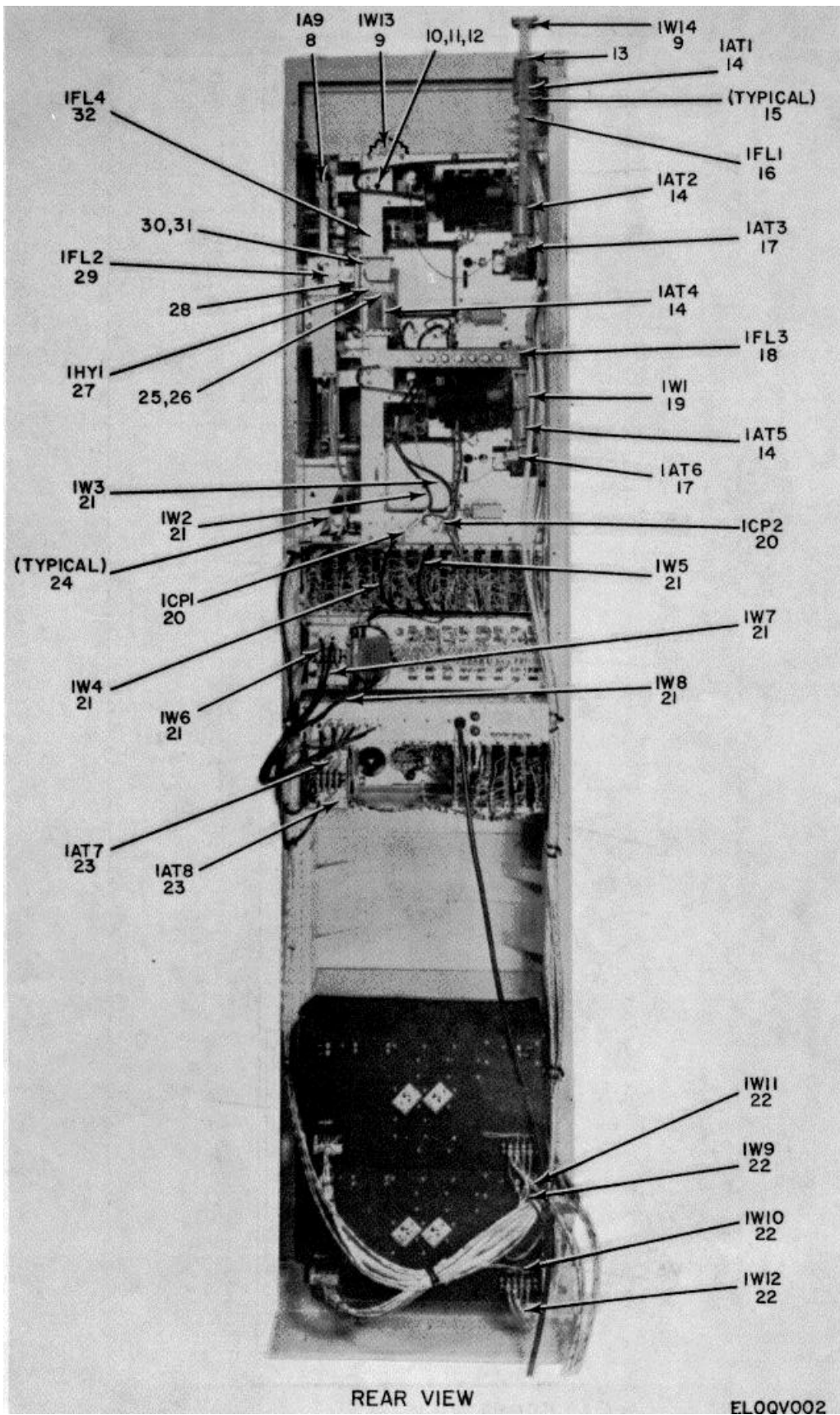
Figure 1. Radio Sets AN/FRC-80(V)1, 2, and 3 (1) (Sheet 2 of 2).
