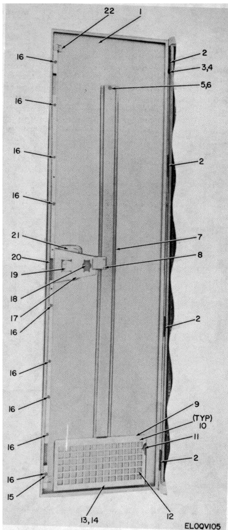
Figure 66. Cabinet, Electrical Equipment CY-7200/FRC (1A11), Door Assembly.
