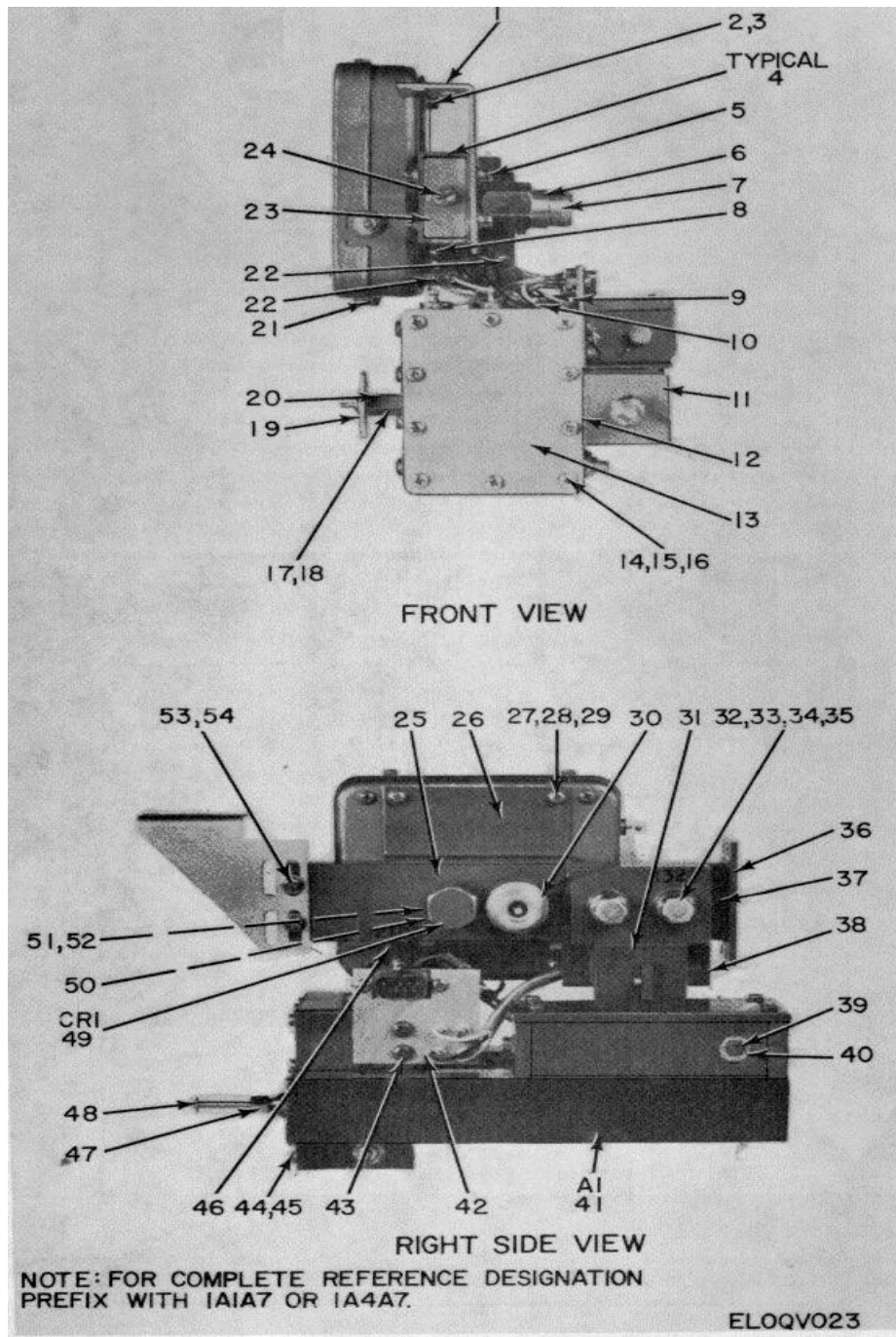
Figure 11. Mixer-Local Oscillator-Preamp (1A1A7) (Sheet 1 of 2).
