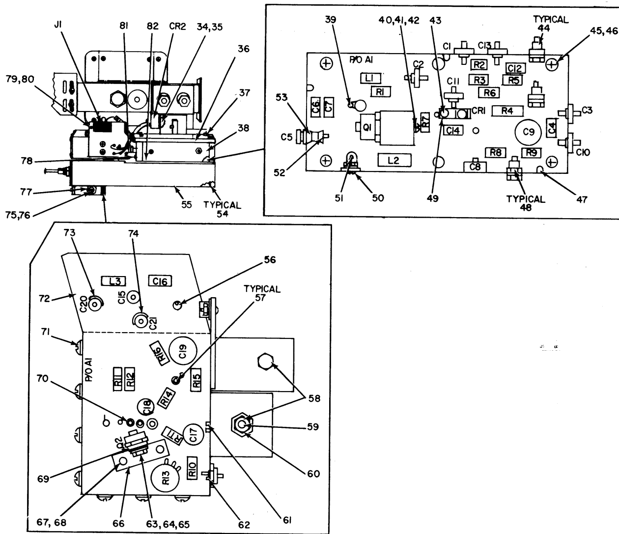
Figure 12. Local Oscillator (1A1A7A1) (Sheet 1 of 2).
