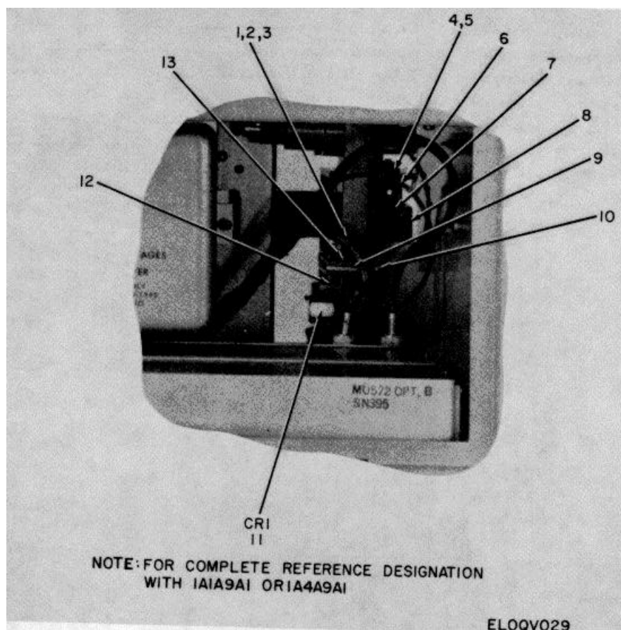
Figure 15. Detector, Frequency Monitor (1A1A9A1).
