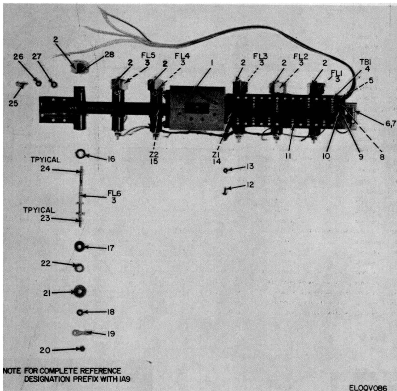
Figure 51. Waveguide Assembly, Transmitter (1A9).
