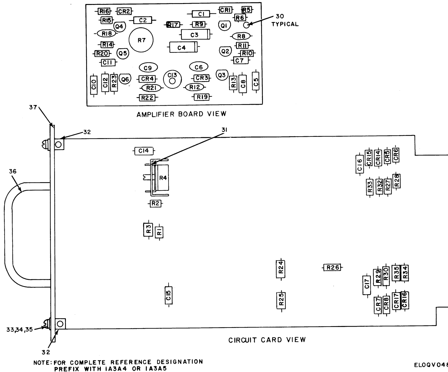
Figure 29. Amplifier, Audio Frequency, Radio AM-6242/FRC (1A3A4) (Sheet 1 of 2).
