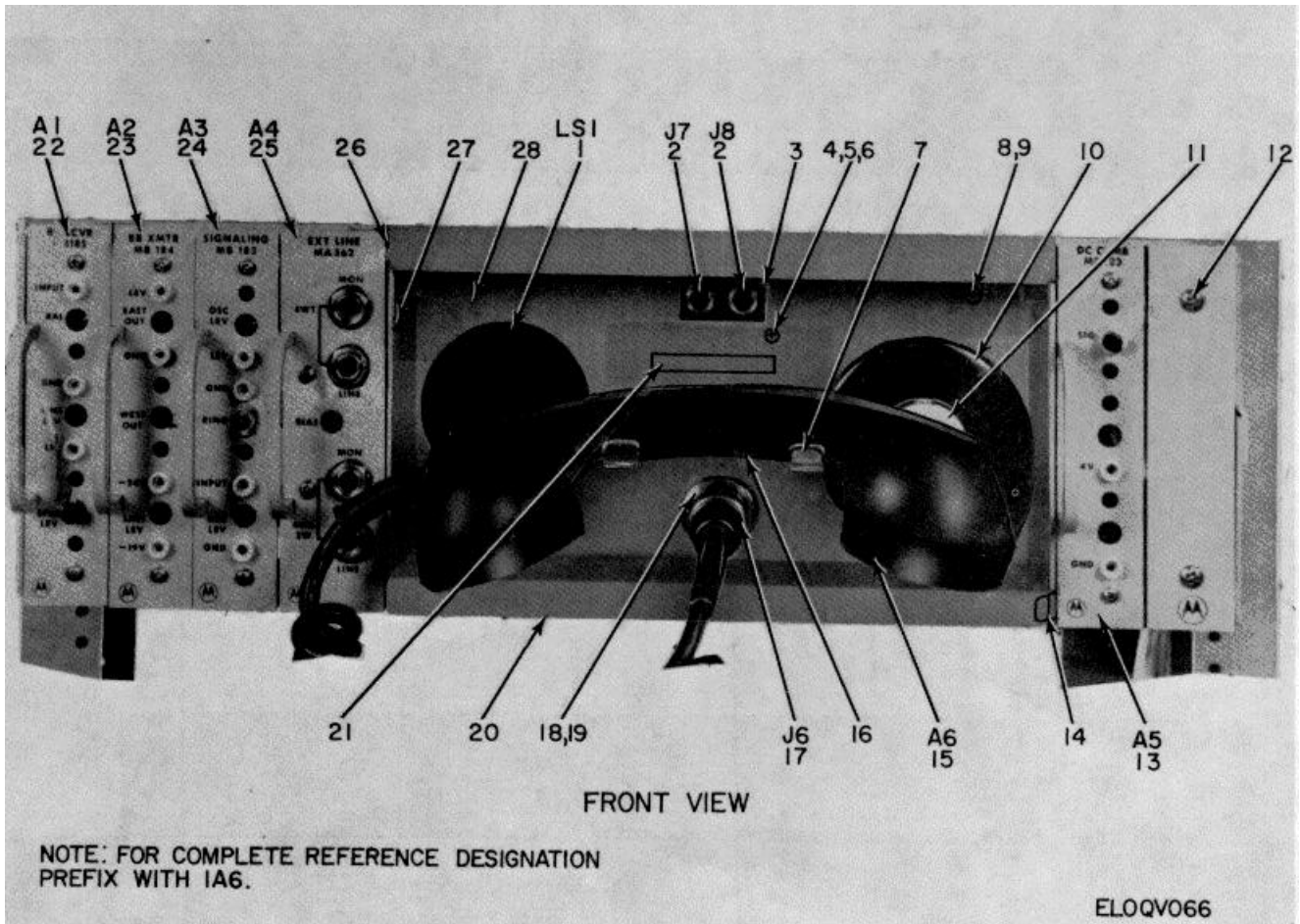
Figure 40. Receiver/Transmitter, Orderwire RT-987(V)1/FRC (1A6) (Sheet 1 of 2).
