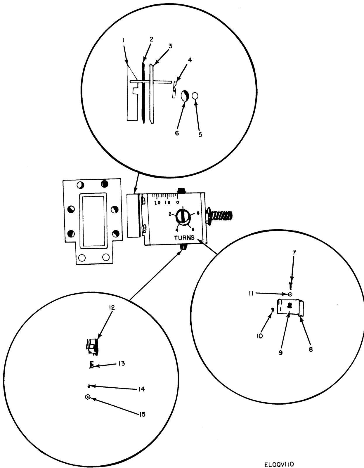
Figure 71. Waveguide and Tuning Assembly (1AT3, 1AT6).
