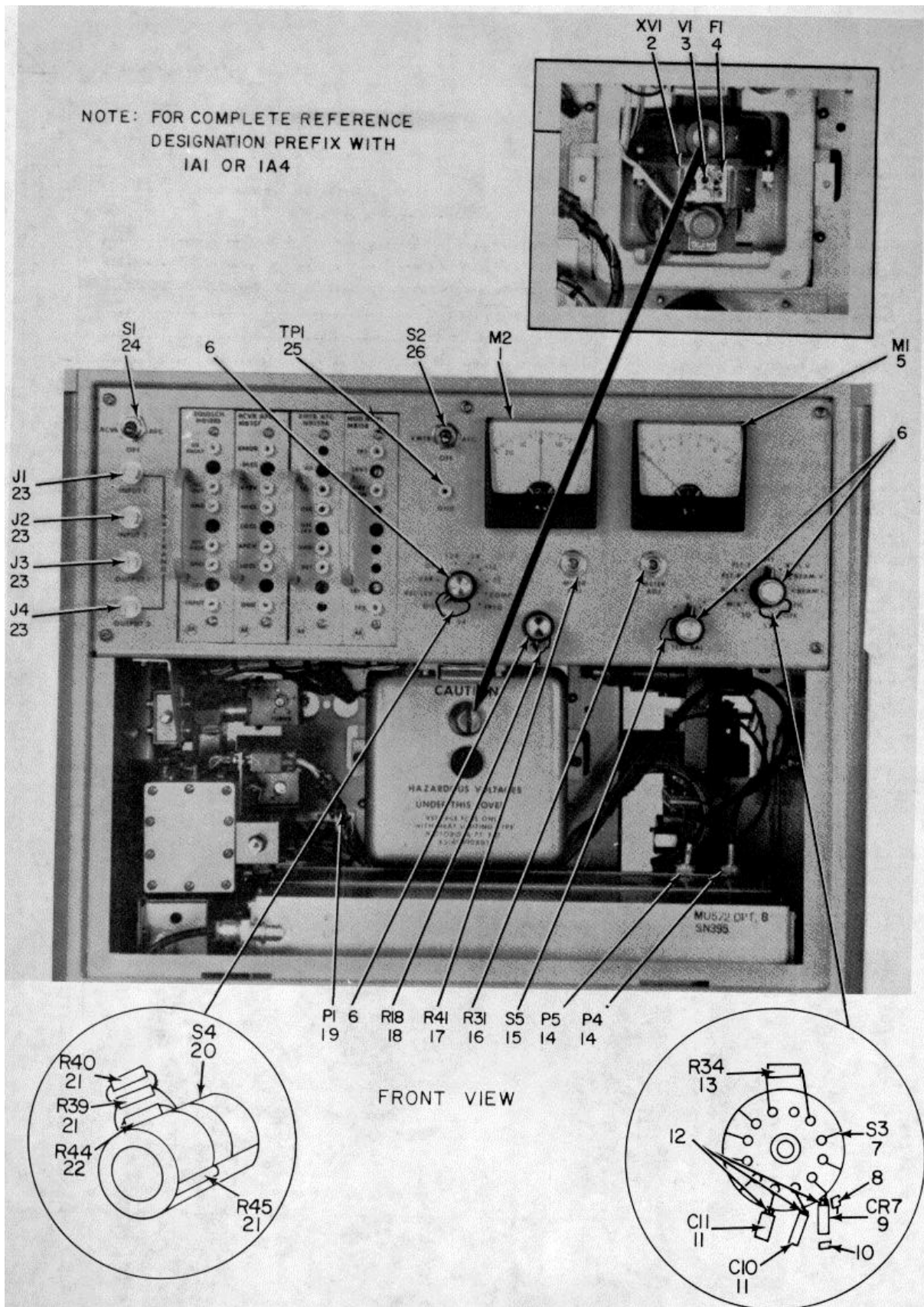
Figure 4. Receiver-Transmitter Radio RT-986(P)/FRC (1A1), Electronic Components Locations (Sheet 1 of 3).
