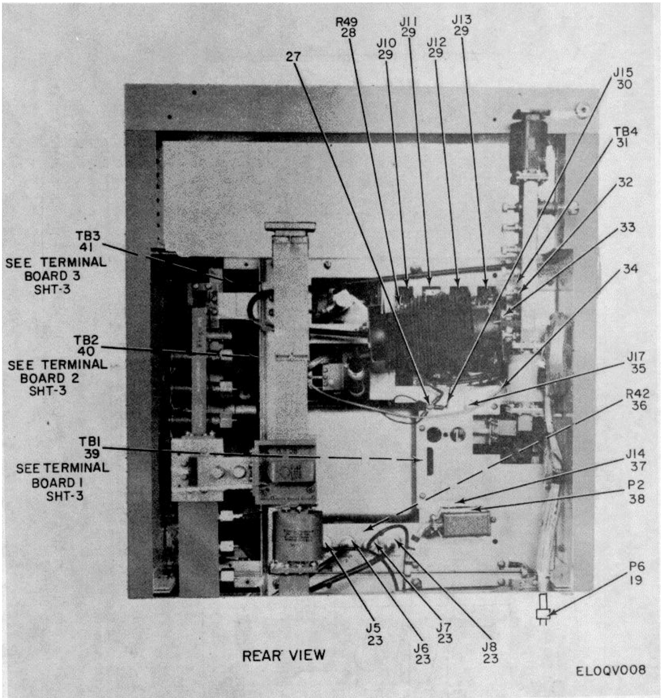
Figure 4. Receiver-Transmitter Radio RT-986(P)/FRC (1A1), Electronic Components Locations (Sheet 2 of 3).
