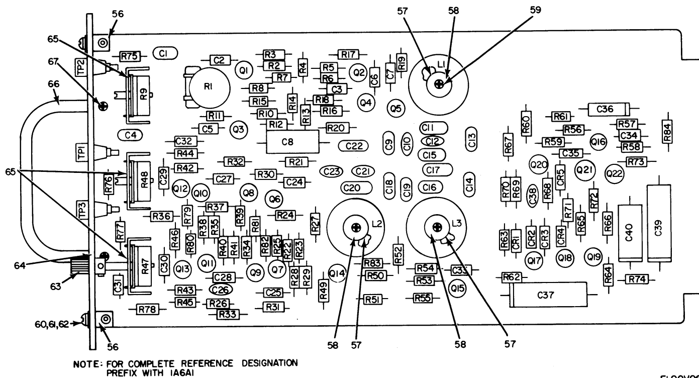
Figure 42. Receiver, Orderwire R-1661/FRC (1A6A1) (Sheet 1 of 3).
