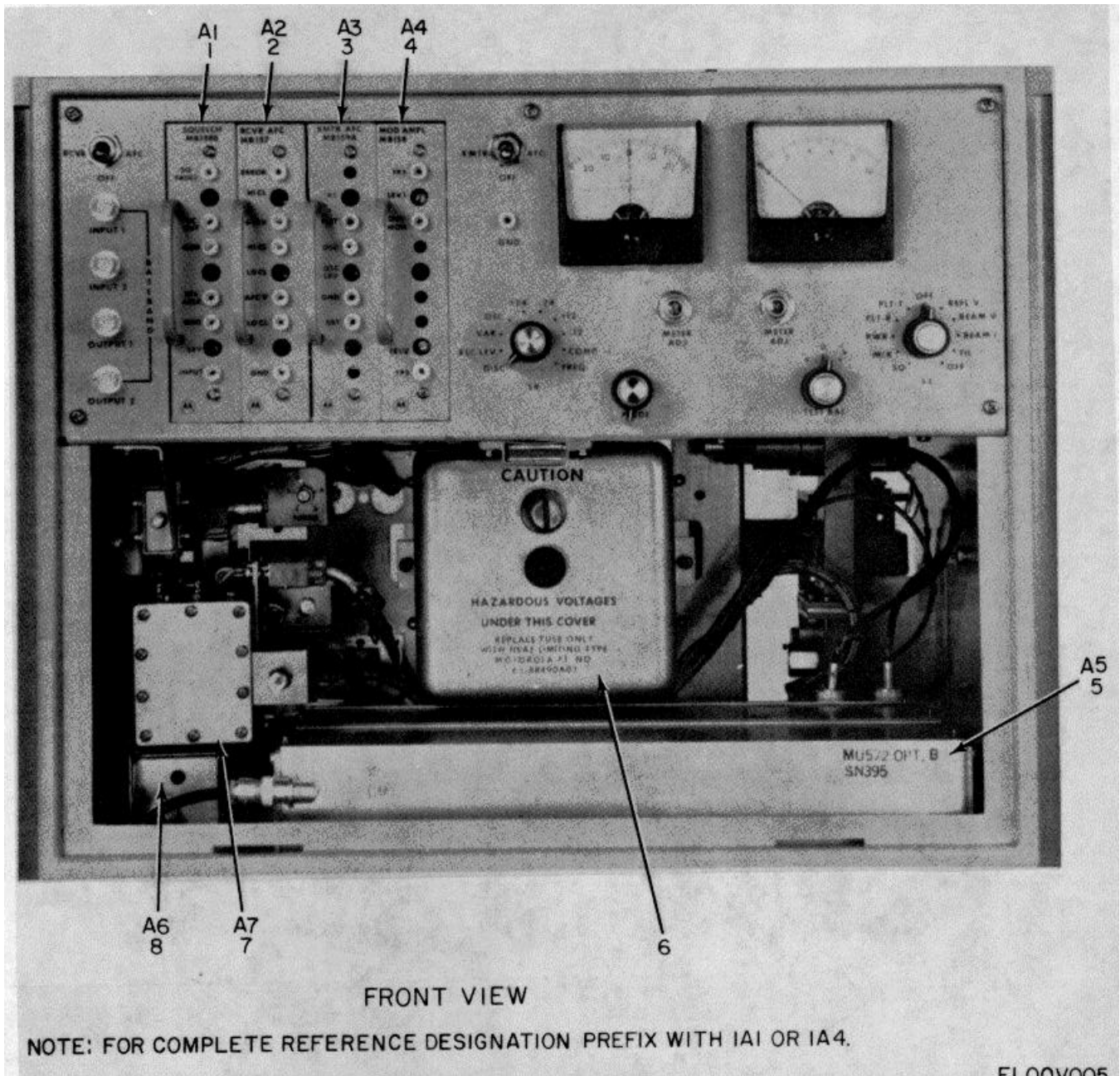
Figure 3. Receiver-Transmitter Radio RT-986(P)/FRC (1A1) (Sheet 1 of 2).
