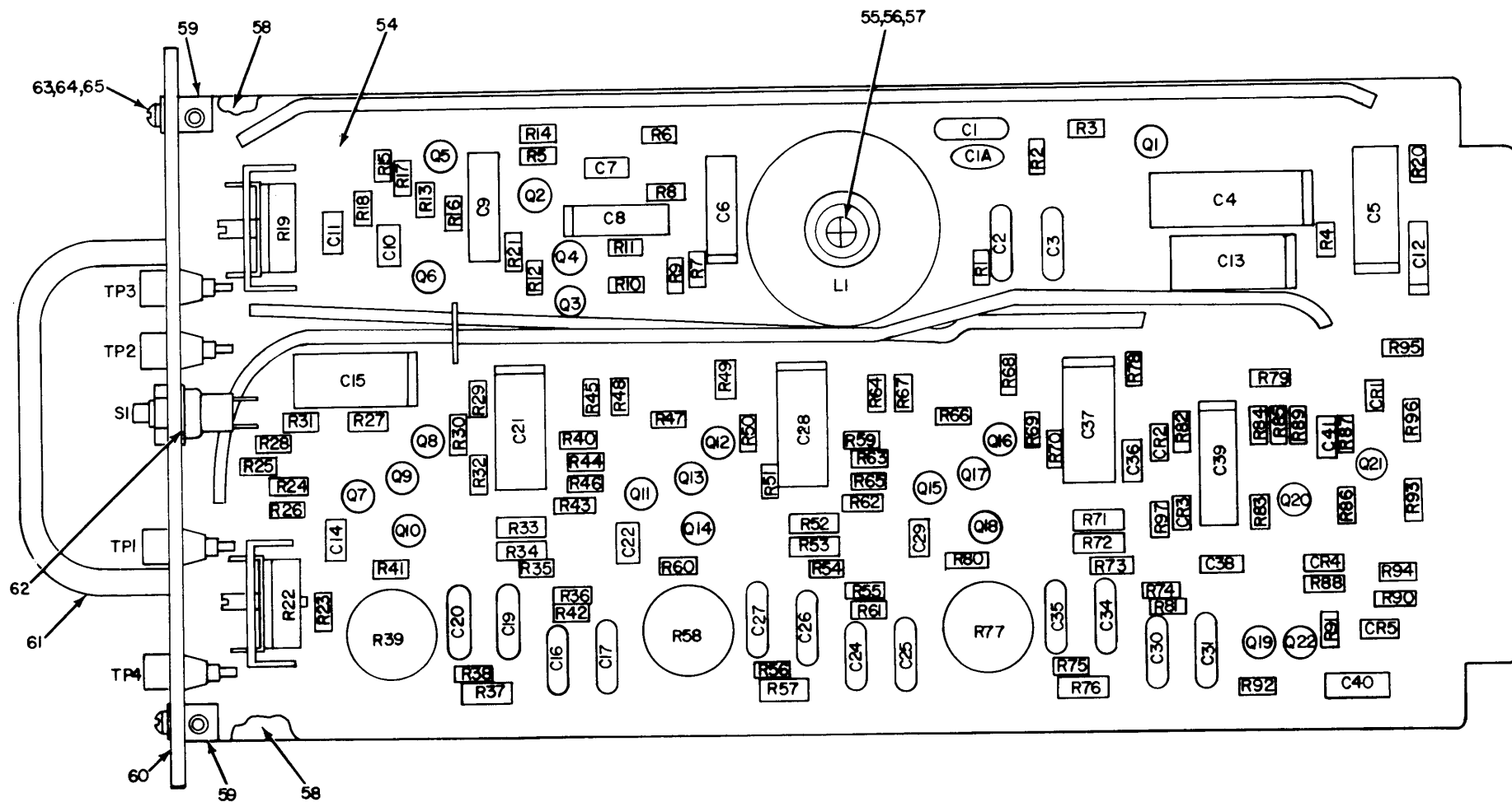
Figure 44. Oscillator, Audio Frequency Signal TA-842/FRC (1A6A3) (Sheet 1 of 3).
