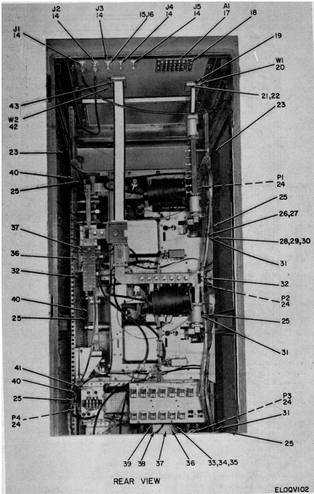
Figure 63. Cabinet, Electrical Equipment CY-7200/FRC (1A11) (Sheet 2 of 2).
