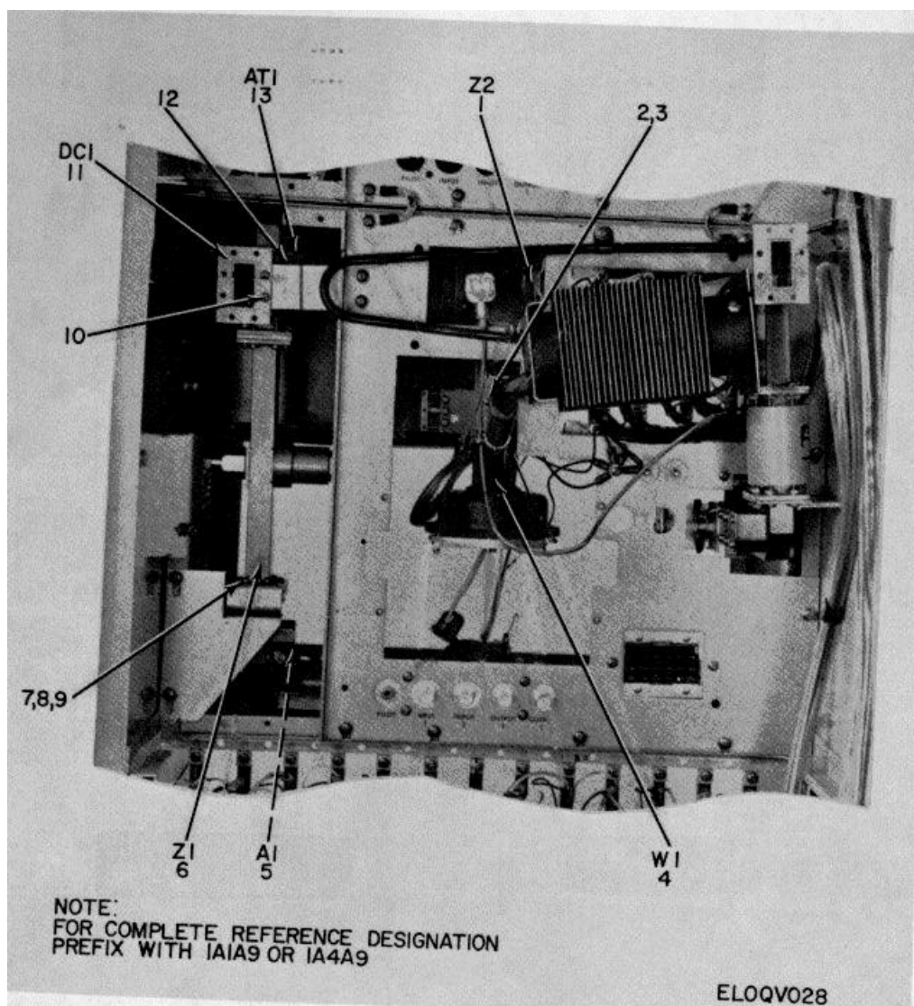
Figure 14. Waveguide Assembly (1A1A9).
