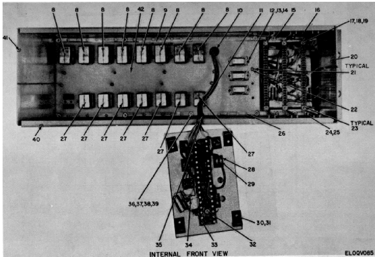
Figure 50. Panel, Combiner Bypass and Alarm SB-3428/FRC (1A7), Mounting Hardware (Sheet 2 of 2).
